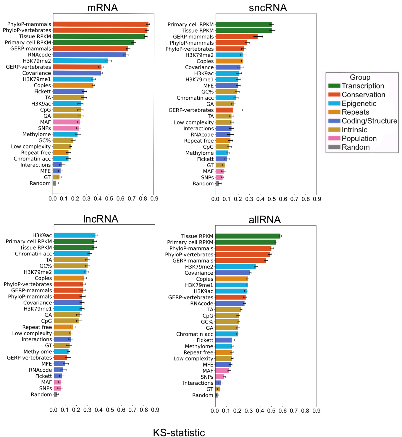
Supplementary Figure S4. Data effect sizes. Features ranked by Kolmogorov-Smirnov (KS) statistic. Each point includes 95% confidence intervals, calculated using bootstrapping (1000 replicates). Different colors represent features groups.
